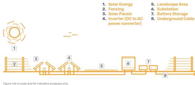
Diagram 2.1 Components of a typical solar PV development
